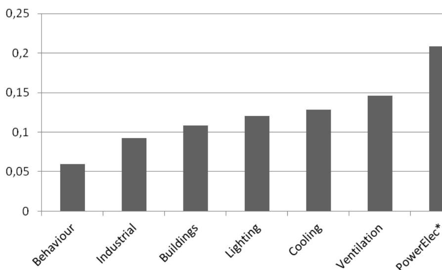
FIGURE 3 - Network density
